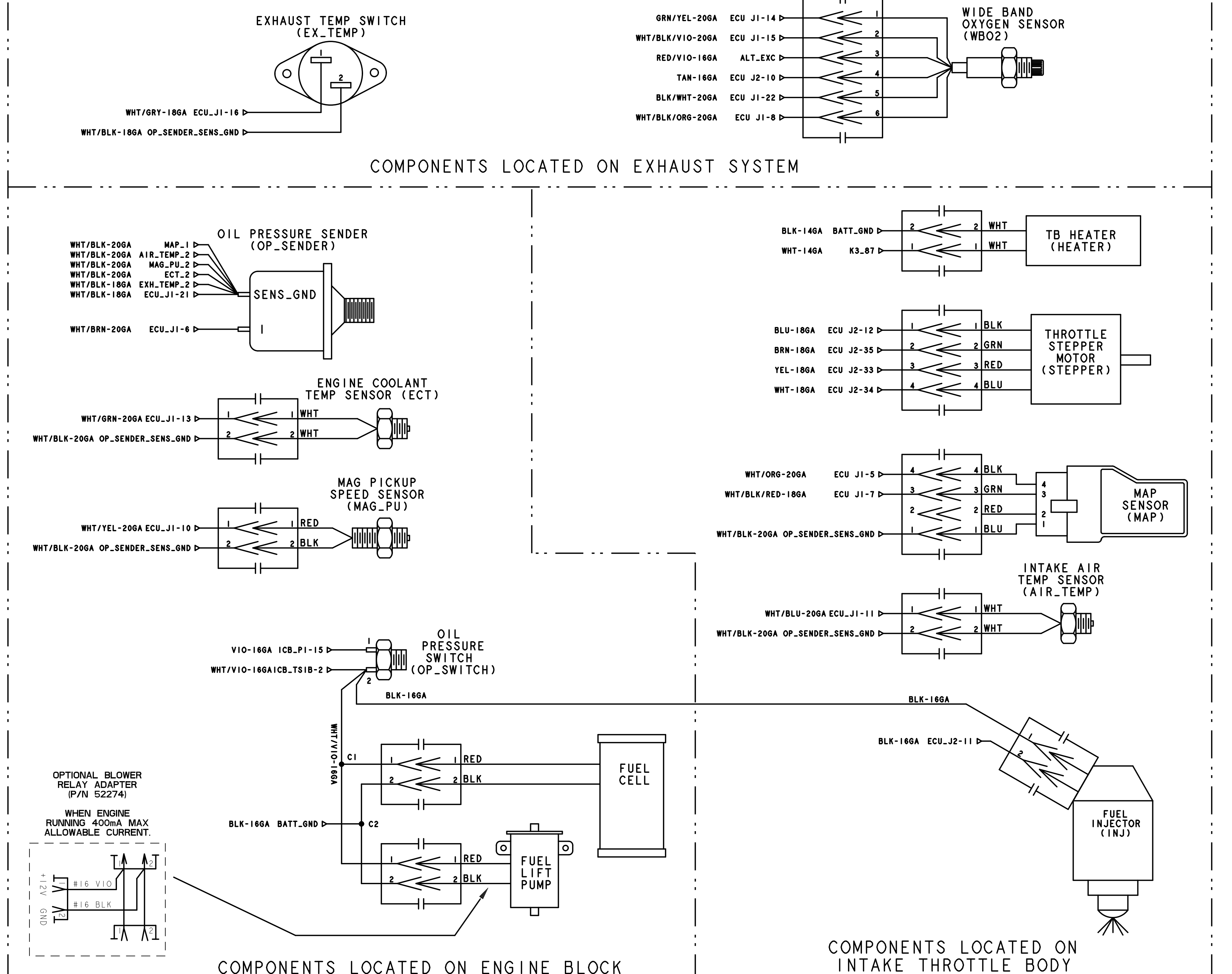
COMPONENTS LOCATED ON ENGINE BLOCK
