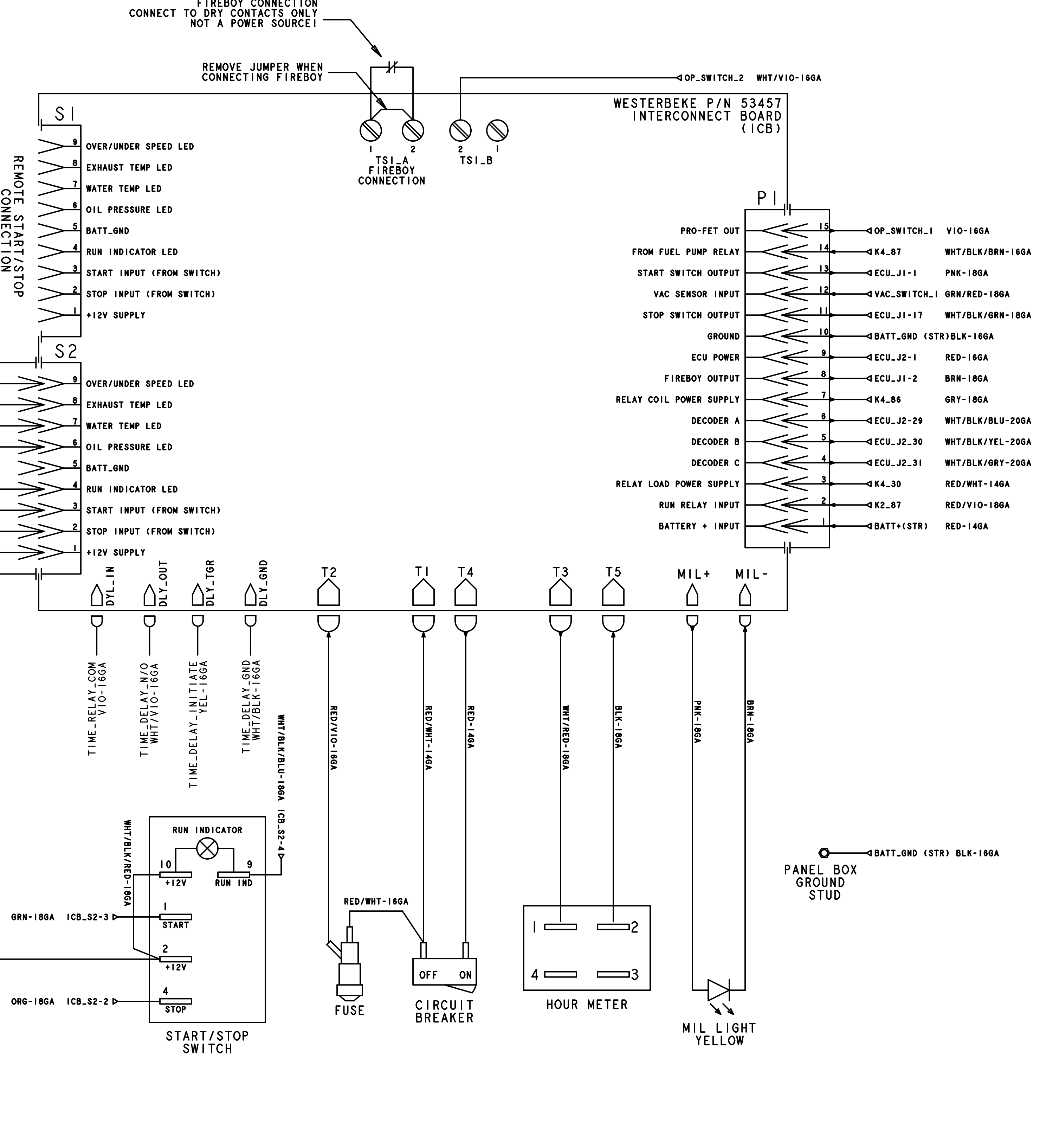
COMPONENTS LOCATED IN CONTROL PANEL BOX
